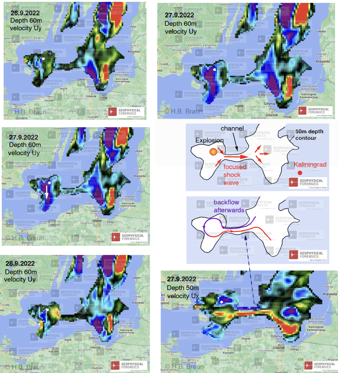
Figure 7 – Underwater canyon and explosion induced underwater vortex formation after the explosion: Left: Satellite images on Sept 26th to 28th (Explosion on Sept 26 at 17:04 UTC) at a depth of 60m. Shown are the North/South components of the currents (yellow/red is directed towards North, blue/black towards South). The white arrow indicates the emergence of a strong underwater current after the explosion away from the detonation site (white dot) which did not exist before (Sept 26th) and considerably after (Sept 28th) the explosion. One should also notice the existence of a pronounced underwater canyon of a width of less than 20km running East West which directly points towards Kalinigrad. On the right hand side both North/South (top) and East/West currents (bottom) are shown at a depth of 50m. Also here red indicates a flow in positive (x or y = East or North) direction, while blue black indicates a flow in the opposite direction. Notice the existence of a significant backflow through the canyon in the aftermath of the explosion compensating the outflow caused by the outgoing shockwave triggered by the explosion. As indicated in the top inset, the shape of the ocean floor near the explosion site (reflecting the Karlskrona bay) had the effect of focussing the shock wave into the underwater canyon giving rise to a highly intense focused shock-wave aimed directly at Kalinigrad and thus explaining the enormous seismic magnitudes in Suwalki. Data Source: GEE: HYCOM satellite images. [Fig7: ©H.B. Braun] .
