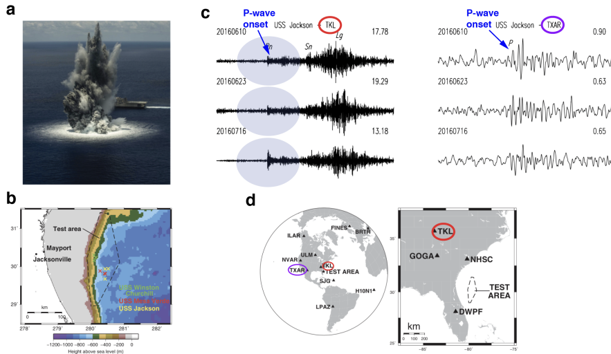
Figure 4 – Comparison to conventional (chemical) underwater explosions ('shock tests' with 10'000 lbs TNT) off the Florida coast: a Conventional explosion triggered by USS Jackson on June 10th 2016, b Location of the explosions c Corresponding waveforms of various tests as registered at TKL (the world's most sensitive seismographic instrument in Tennessee under DoD management) and TXAR (Texas). Note the similarity to the earthquake in Fig 5 and the striking difference to the nuclear event shown in the same Figure. Source: R. Heyburn, S.E. J. Nippres, and D. Bowers, Seismic and Hydroacoustic Observations from Underwater Explosions off the East Coast of Florida , Bull. Seism. Soc. Am. 108 , pp. 3612–3624, (2018). [Link]
