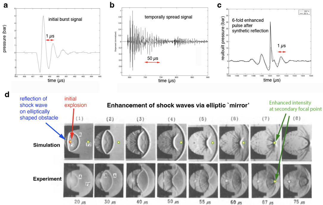
Figure 8 – Focusing effect of shockwaves a - c The dispersion of a sharp detonation signal can be reversed through reflection. In this example an initial burst signal of 1 \mu\text{s} duration is spread to 50 \mu\text{s} in a waveguide. In this example of a piezo-dispersive generator the electronically simulated reflection ('time reversal mirror') recreates a shock wave c whose pressure amplitude exceeds that of the original pulse by a factor 6. [Reference: S. Dion, C. Herbert, M. Brouillette, Comparison of method for generating shock waves in liquids , in Shock Waves, eds Hannemann Seiler, 26th Symposium on Shock waves, 2007, Springer (2009)]. d Focusing of shock waves in water via an elliptically shaped boundary: A shock-wave that is created at the detonation point (orange/red) bouncing off the elliptically shaped reflector (black, left) and upon reflection becomes focussed close to the green/yellow focal point with maximal focussing at the instant of image (7) (2nd last column). Notice the similarity to the shape of the ocean floor close to the detonation point (cf. Fig. 7, top inset). Thus after reflection at the underwater basin a secondary shock wave is generated and directly focussed into the entrance of the underwater Canyon directed at Kaliningrad. [Reference: K. Isuzugawa, M. Horiuchi, Experimental and numerical studies of blast wave focusing in water , in "Shock Waves", Proceedings Sendai 1991, Vol1, Springer (1991).]
