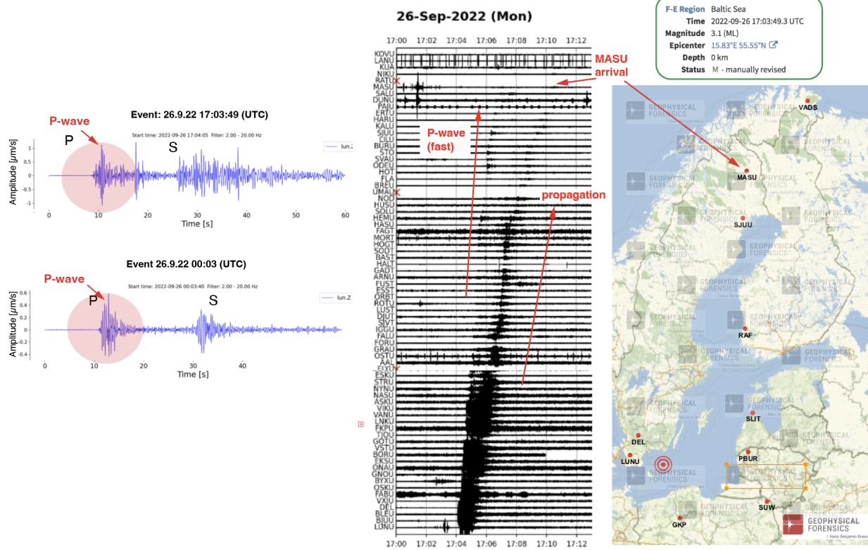
Figure 2 – NordStream explosion and seismic signatures at Swedish stations according to the website of the Swedish Seismological Service SNSN [5] [Most of the data displayed in Ref. [5] are not available as waveforms and thus can not be analysed]. Left: Seismic waveforms measured in Lund (LUNU: 55.63200°, 13.44680°) the first (weaker) event around midnight on Sept 26, and a stronger event at 17:03 (UTC). Note the sharp rise of the P-Wave signal whose amplitude exceeds that of the subsequent shear waves. Middle: Propagation of the seismic waves towards North, where station MASU is the most northern Swedish station displaying seismic signatures which is at a distance of 1365km from the explosion site (the Norwegian station VADS at 1754km also displays seismic signatures of the 17:03 event, and in fact also stations in Iceland and Greenland). Inset top right: Entry in the Geofon database describing the localisation of the explosion up to 8km. This "Geofon Global Seismic Monitor" indicates magnitude M_L = 3.1 for the event at 17:03:49.32 (UTC). Source: [10] ([Link]).
