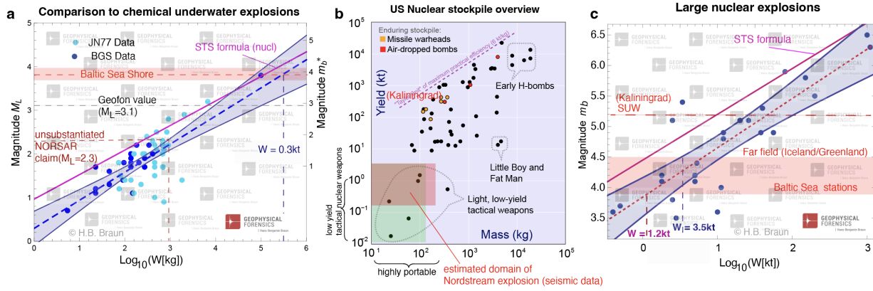
Figure 1 – Relation between magnitude m_b and the TNT mass equivalent for chemical underwater and nuclear detonations: a , Chemical underwater detonations according to data by the British Geological Survey (BGS) [18], [Link], also including data by Jacobs and Neilson (JN77) with the 'depth optimized' events omitted as they are irrelevant in the current context. a Here the Richter magnitude M_L and regional magnitude m_b^* are plotted against \log_{10}(W) with W the detonation energy measured in kg TNT equivalents. The broken line is the linear regression through the data points with the shaded area indicating the 95% confidence interval. The violet straight line is the STS expression of Eqn (1), m_b = 4.45 + 0.75 \log W (cf. C. Ammon et al. Found. of Mod. Global Seismology , Ass. Press, 2nd ed. 2021). The red-shaded area results from the magnitude derived from the waveform amplitudes in the Baltic Sea area resulting in an estimate for the explosive charge energy of 0.2 kt ( 1 \text{ kt} = 10^6 \text{ kg} ). Note that the STS relationship provides essentially a lower bound on the explosive charge at a given magnitude ( M_L or m_b^* ) for all collected data presented here, b , Overview over the US nuclear stockpile (Wiki). The green shaded area marks the range of (thermonuclear) tactical nuclear weapons with W in the range of 10 tons (t) up to several kilotons (kt) with an actual physical weight in the range of less than 100kg that can be transported even with underwater unmanned vehicles (UUV) (cf. NATO Repmus"22 exercise, Sept 12-22, 2022 [14] ([Link])). c , Magnitude explosive-charge relationship for nuclear explosions listed in the BGS report [18]. The broken line is the linear regression with the shaded area denoting the 95% confidence interval. Notice that here the charge is measured in kilotons. The red shaded areas denote estimates that result from seismic considerations, lower band extending from Baltic Sea to magnitudes derived from waveforms detected in Greenland/Iceland ( m_b = M_S \approx 4.5 ). The upper value results from the vicinity of Kaliningrad ( m_b^* \approx 5.2 ). Based on the STS relationship, the resulting values for the explosive charge are between W = 0.2 \text{ kt} and 4 \text{ kt} (the considerable uncertainty is due to the logarithmic dependence). It should be noted that the enormous values of the seismic magnitude near Kaliningrad are due to shock wave amplification via the underwater canyon as shown in Fig. 7. [Fig1a,c: ©Hans-Benjamin Braun]
