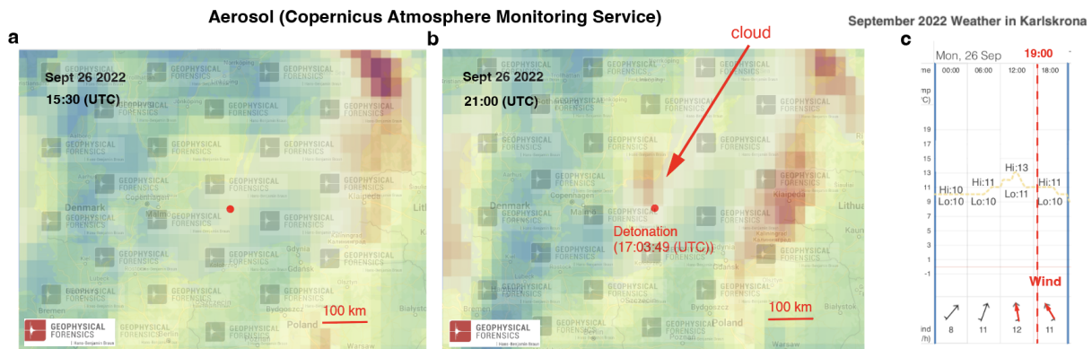
Figure 6 – Aerosols both before and after the detonation: a, Aerosol distribution 1.5 hours before the detonation detected in the infrared at 785nm wavelength. b, Aerosol distribution 4 hours after the detonation (note that local time = UTC +2) . Clearly visible are both the extended cloud emanating from the detonation site (red dot) into the direction of the prevailing winds (cf. c) and extending over 100km. Also clearly visible is the enhancement of the aerosol concentration along the Kaliningrad coastline as is expected from the focussing of shock waves along the underwater canyon directed at Kaliningrad (cf. Fig. 7) and the entailing enormous seismic magnitudes observed at Suwałki in the border region of Belarus, Lithuania, Poland and Kaliningrad. c Wind direction in Karlskrona on the Swedish coast facing the explosion site against the wind direction. [Source: GEE: Copernicus Atmosphere Monitor (CAMS) @ 785 nm wavelength]. [Fig5a,b: ©H.B. Braun]
