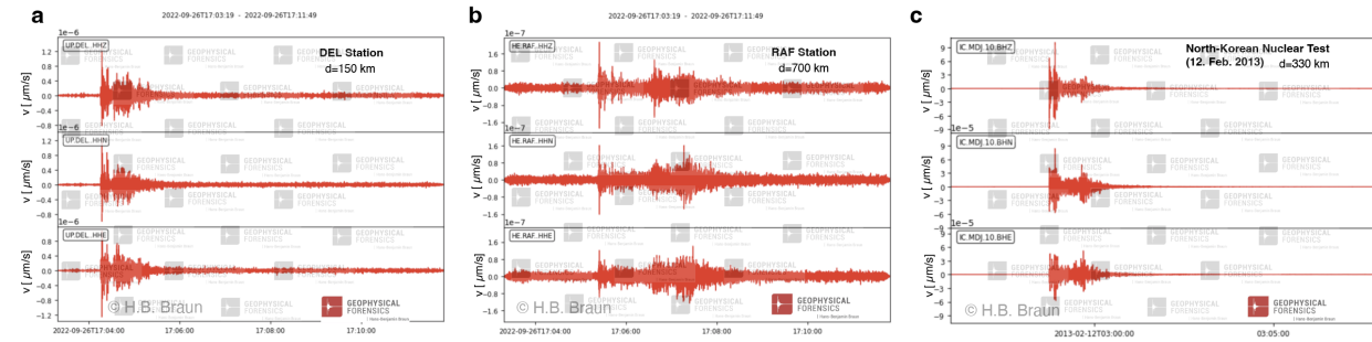
Figure 3 – Measured 3D seismograms of DEL and RAF compared to a North-Korean underground nuclear test of magnitude M_L = 5.1 . a , Measured seismic response at DEL on the Swedish mainland at a distance of 150km towards West (cf. Fig. 2). From top to bottom: Response in vertical (Z), north (N) and East (E) direction. Notice the abrupt beginning of the response which is characteristic of a shock wave which is particularly pronounced for a nuclear explosion. Also characteristic for an underground event is the nearly isotropic response indicating the existence of a hybrid water/solid shock primary wave. b , Measured response at the station RAF situated at the Finnish coast close to Turku at a distance of 700km. Also here the onset of P-waves is still well pronounced. Note that the station RAF is virtually freely accessible across water from the detonation site. For this reason the shock wave arrives virtually unscattered and is moving with a velocity of approx. 6 km/s far exceeding the sound velocity (1.5km/s). Note both panels a and b reveal a periodic substructure which is related to resonance-like reflection of shock waves in coastal regions. c , Measured response of a underground nuclear test (UNE) in North Korea of strength M_L = 5.1 corresponding approx. to a 7 kt TNT yield. Clearly visible are the clear onset of the P-wave which also exceeds the intensity of the surface waves. [Note, based on the independent method employed here, the same estimate M_L = 5.1 was obtained determined in the following press release of the Earth Institute of Columbia University [Link]]. [Fig3a,b: ©H.B. Braun]
